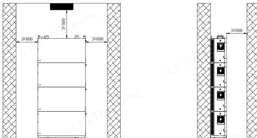
Installation distances from adjacent objects
